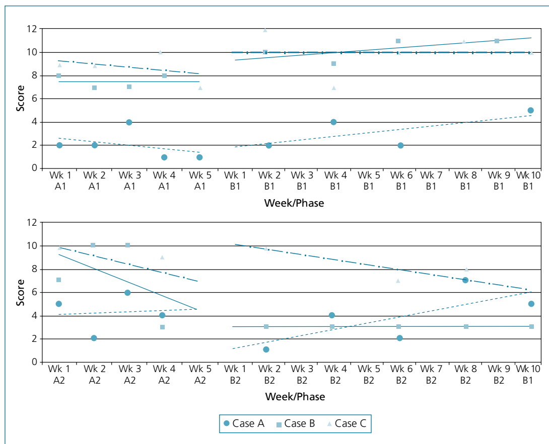
Figure 1. Sensory Over-Responsivity scales—positive behaviours
