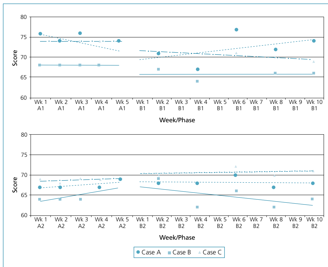
Figure 3. Sensory Processing Measure—auditory sensory processing subtest (HEA)
